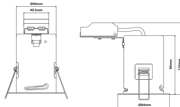
IP65 Showerlight : Bezel Diameter 86mm Cut-Out: Ø69mm
