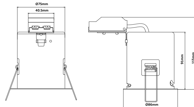
Centre Tilt: Bezel Diameter 86 mm Cut-Out: Ø78mm
