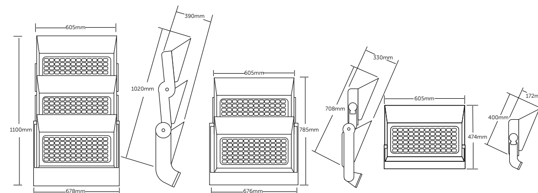
Dimensions include optional Deep ULR Shields
