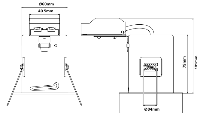
Fixed: Bezel Diameter 84mm Cut-Out: Ø68mm
